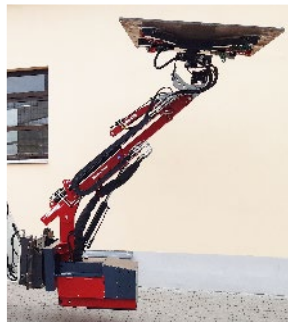
Various adapters (e.g. Euro mount) possible for simple and uncomplicated mounting on various work machines such as telescopic handlers, etc.
