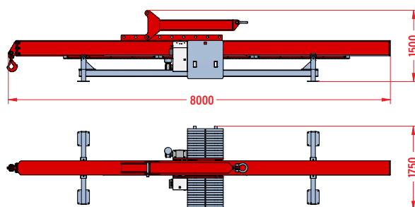
Mounting Frame Technical Data (mm)
